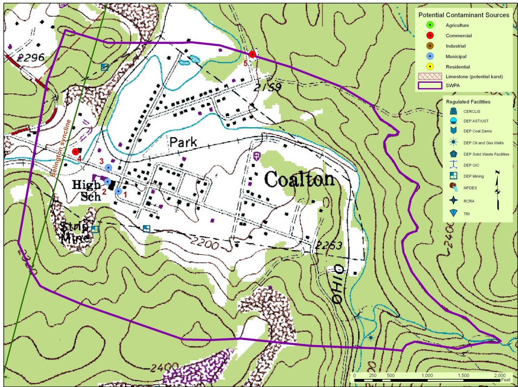
Figure 1: Coalton Water System Source Water Protection Area
