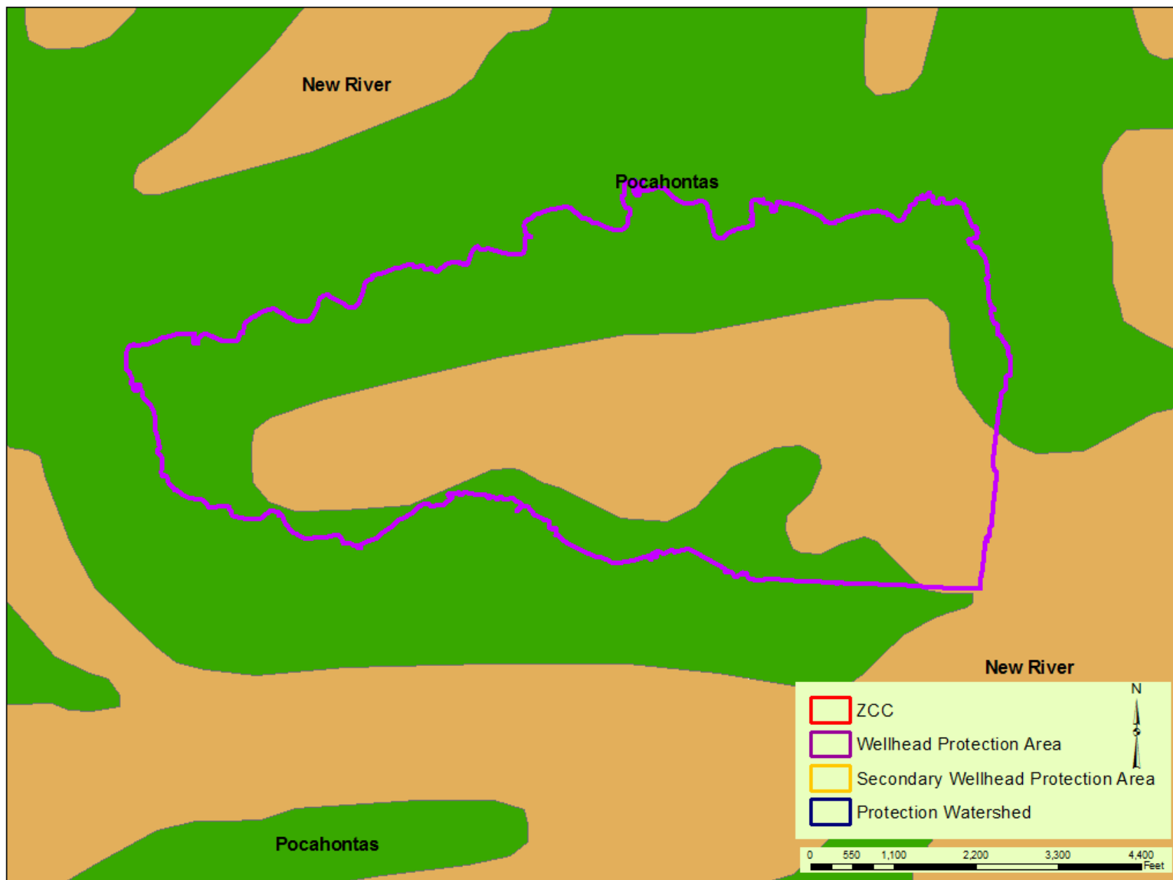
Figure 5 McDowell County PSD Greenbrier Geologic Map
